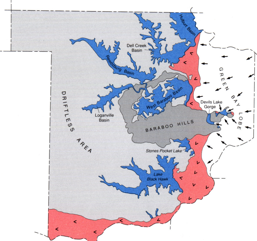
Major geologic features of Sauk County during the maximum late Wisconsin extent of the Green Bay Lobe. The map shows the location of the western edge of the Green Bay Lobe (arrows show direction of ice flow), outwash plains (red), and lakes (blue). The Baraboo Hills and the remainder of the Driftless Area in Sauk County are shown in shades of gray.
